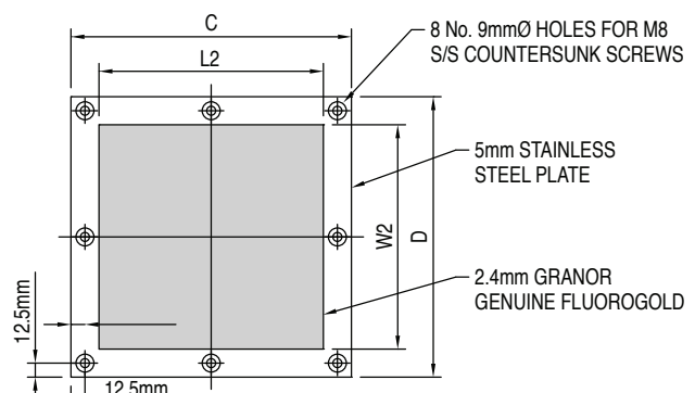
PLAN VIEW – BOTTOM ELEMENT
