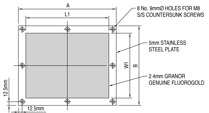
PLAN VIEW – TOP ELEMENT (VIEW FROM UNDERSIDE)
