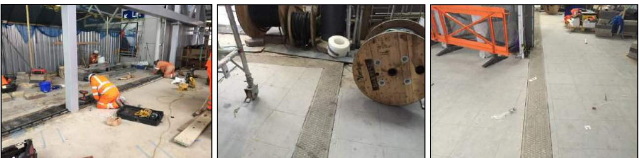
Ekspan T-Mat 80 Expansion Joint installed in Leeds Station – Southern Entrance.
