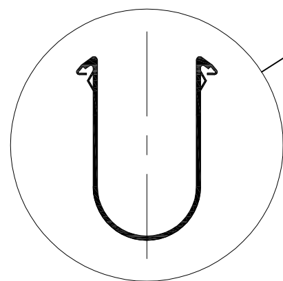
ALTERNATIVE DRAPE SEAL
