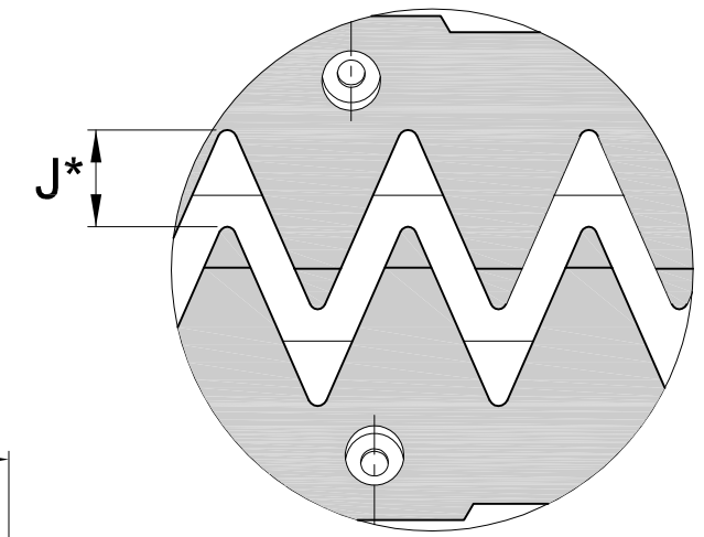
PLAN VIEW FINGER GAP
